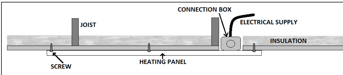
FIGURE 1 – Surface Mounting
